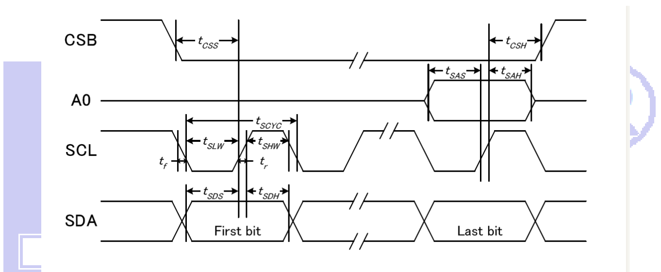
图 3. 从 CPU 写到 ST75256 (Writing Data from CPU to ST75256)
